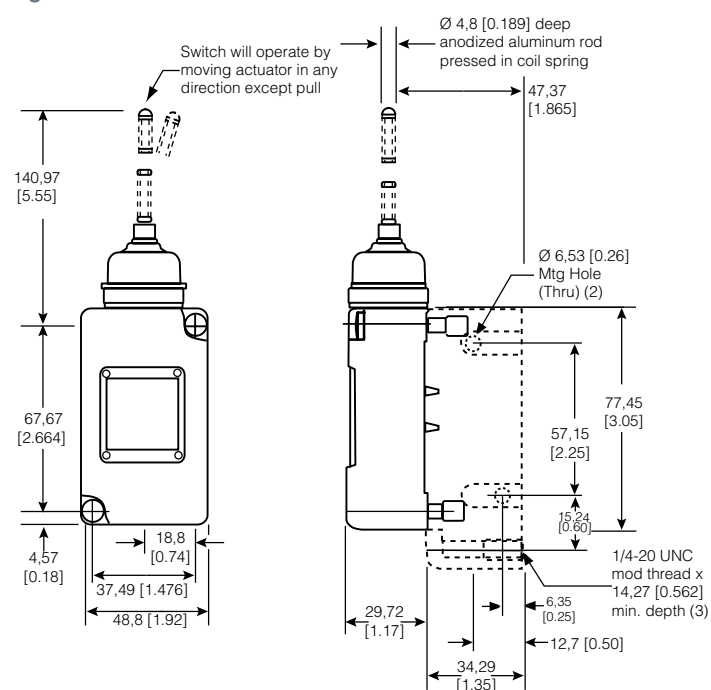
Figure 21. 208LS3 Dimensions
