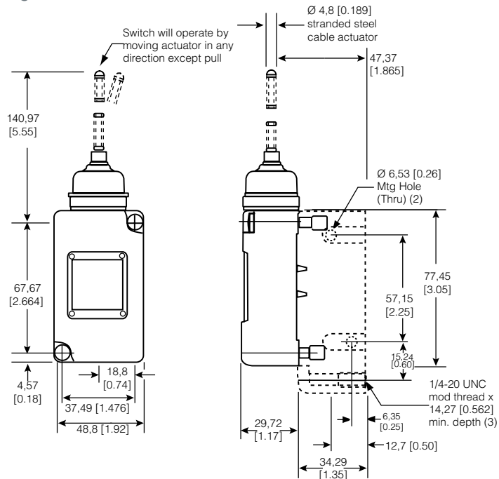
Figure 20. 208LS1 Dimensions
