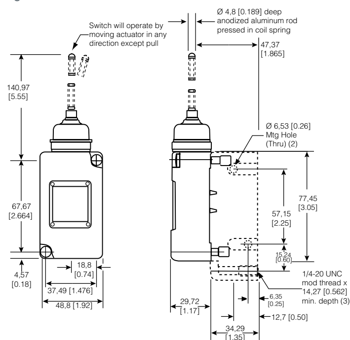
Figure 21. 208LS3 Dimensions
