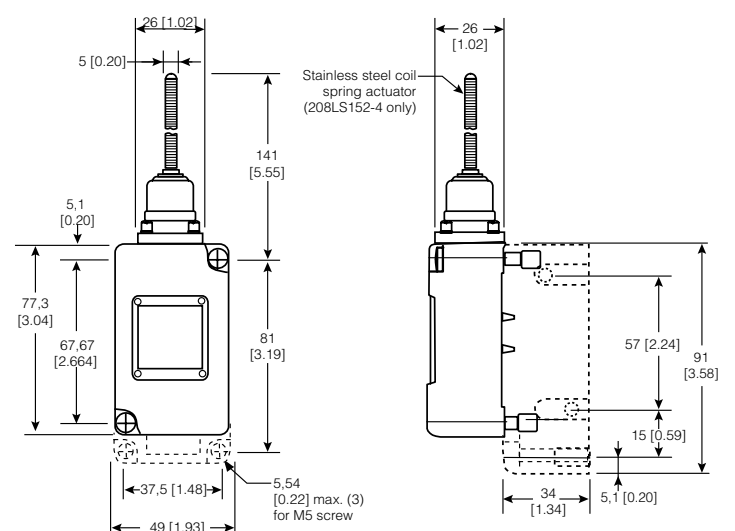
Figure 39. 208LS1-4 Dimensions
