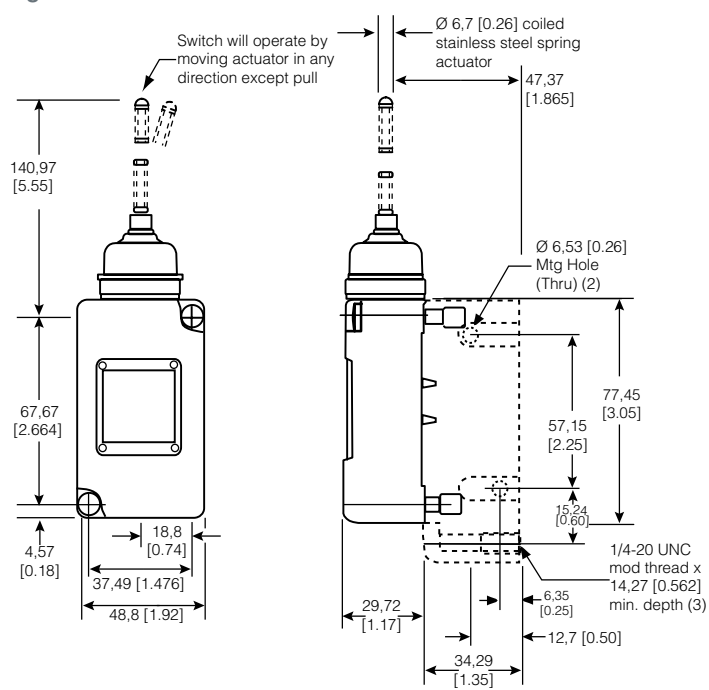
Figure 23. 208LS152 Dimensions
