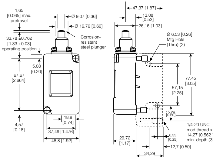
Figure 15. 202LS1 Dimensions
