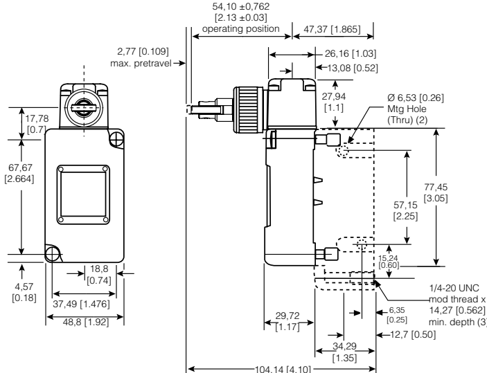
Figure 16. 203LS1 Dimensions
