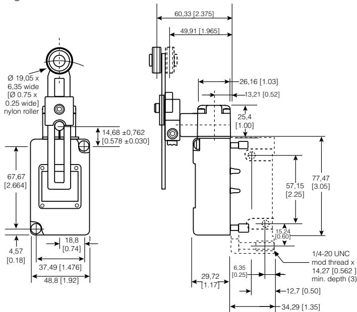
Figure 13. 201LS3 Dimensions
