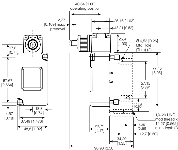
Figure 18. 205LS1 Dimensions
