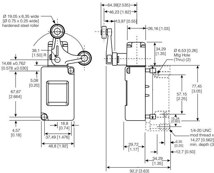
Figure 19. 206LS1 Dimensions
