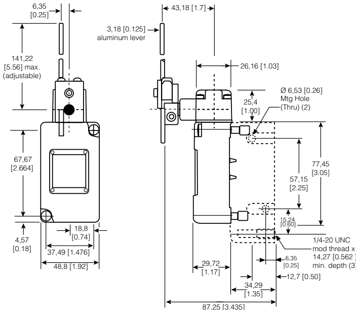
Figure 15. 202LS1 Dimensions
