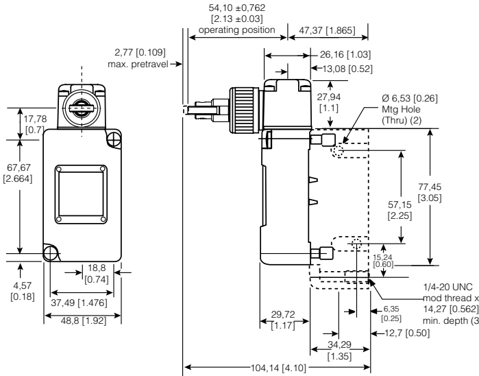
Figure 16. 203LS1 Dimensions
