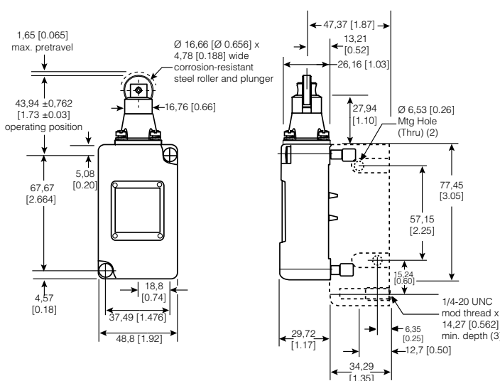
Figure 19. 206LS1 Dimensions
