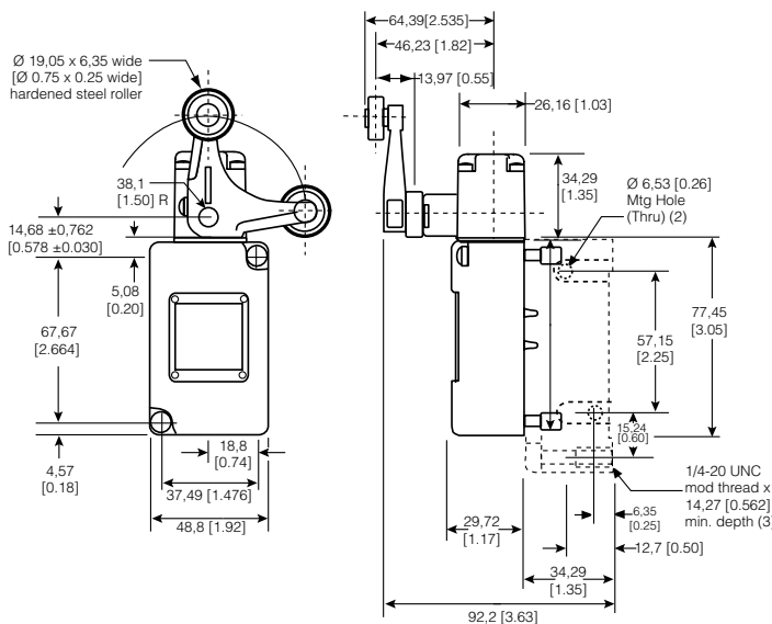
Figure 19. 206LS1 Dimensions
