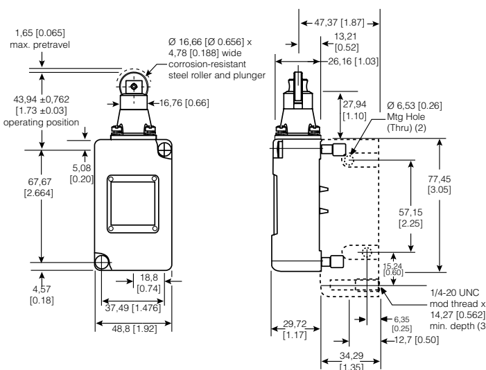
Figure 19. 206LS1 Dimensions
