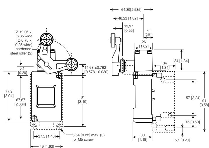
Figure 34. 201LS3-4 Dimensions
