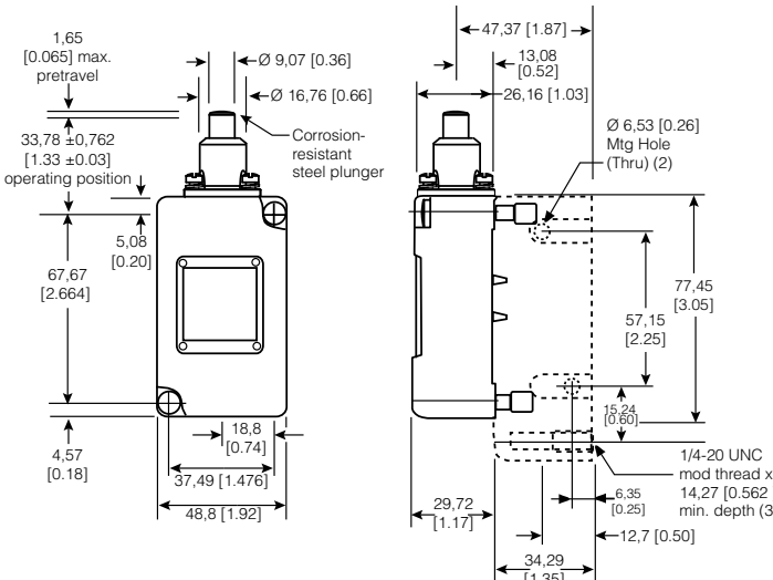
Figure 16. 203LS1 Dimensions
