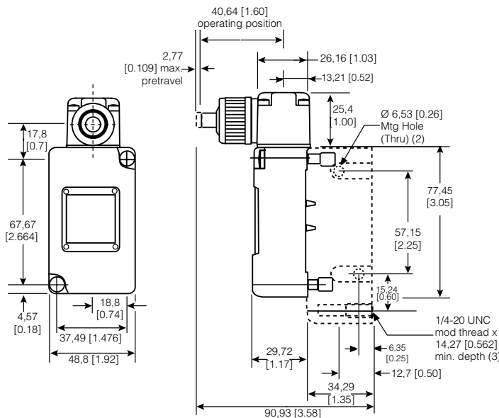
Figure 18. 205LS1 Dimensions
