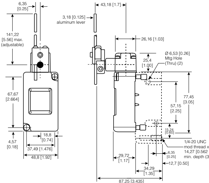
Figure 15. 202LS1 Dimensions
