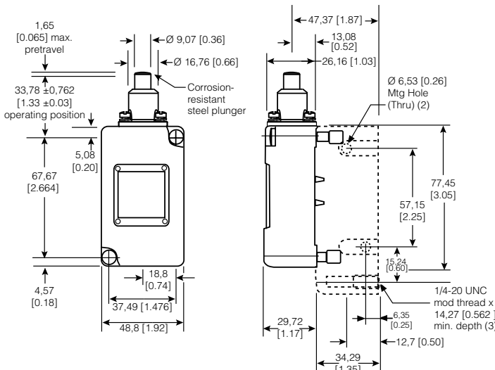
Figure 16. 203LS1 Dimensions
