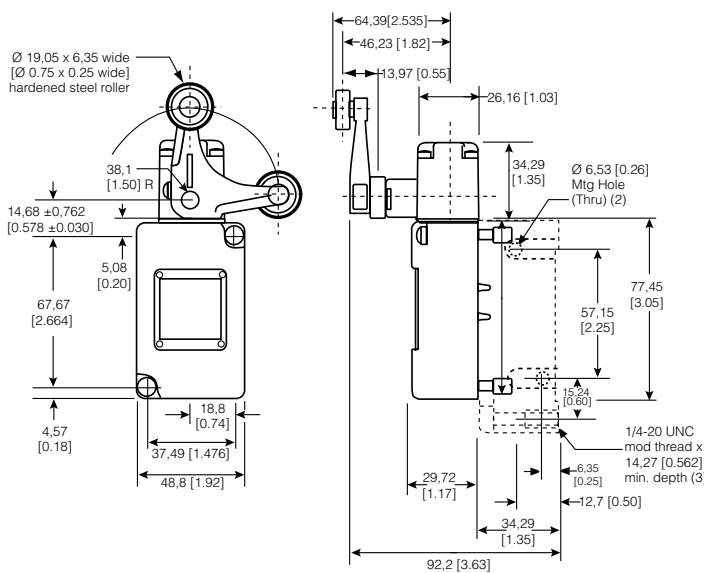
Figure 19. 206LS1 Dimensions
