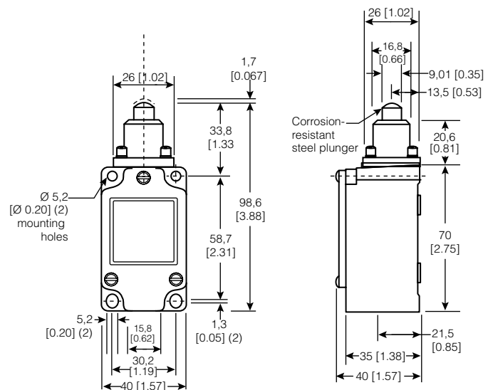
Figure 28. 4LS1-4 Dimensions
