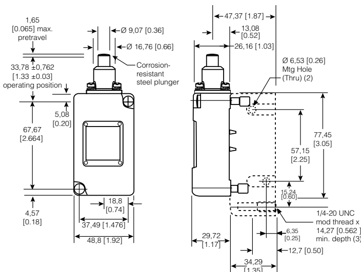
Figure 16. 203LS1 Dimensions
