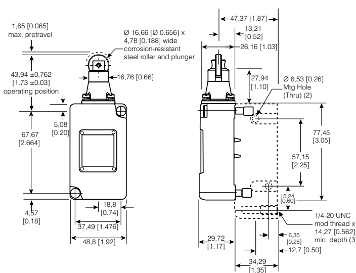
Figure 19. 206LS1 Dimensions
