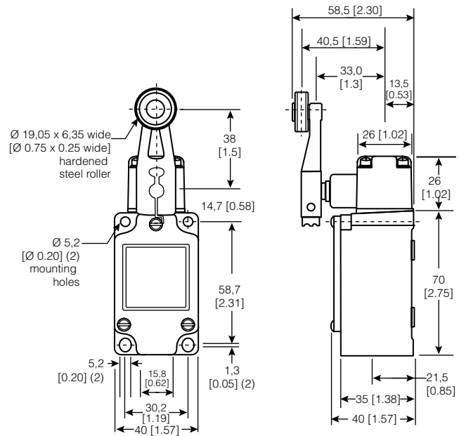
Figure 27. 2LS1-4 Dimensions
