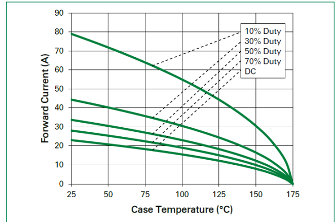
Figure 4: Current Derating
