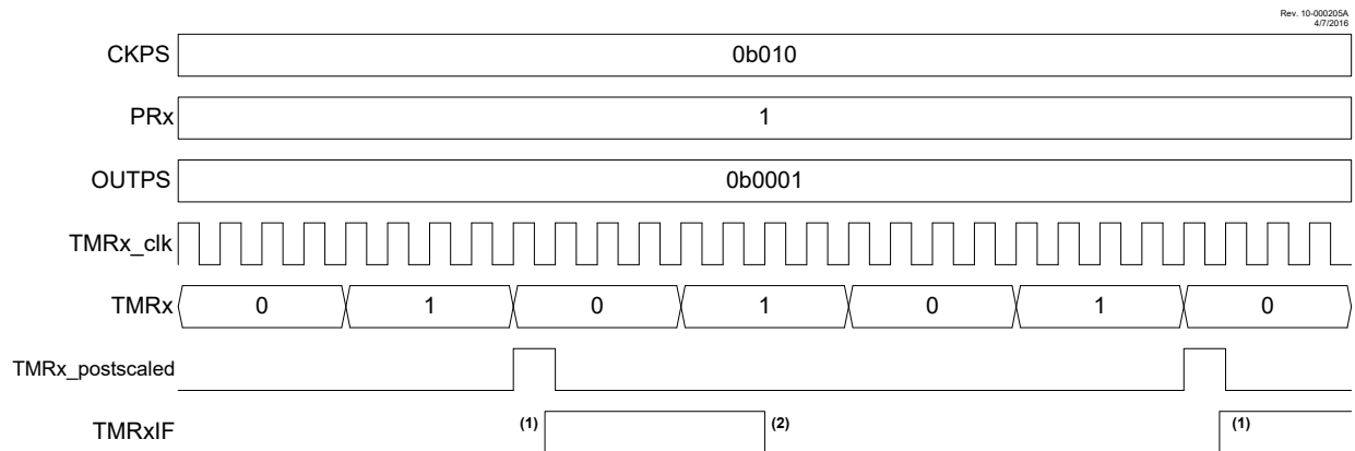
Figure 20-2. Timer2 Prescaler, Postscale, and Interrupt Timing Diagram
