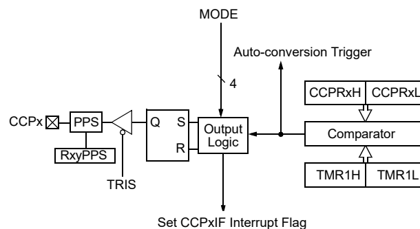
Figure 21-2. Compare Mode Operation Block Diagram
