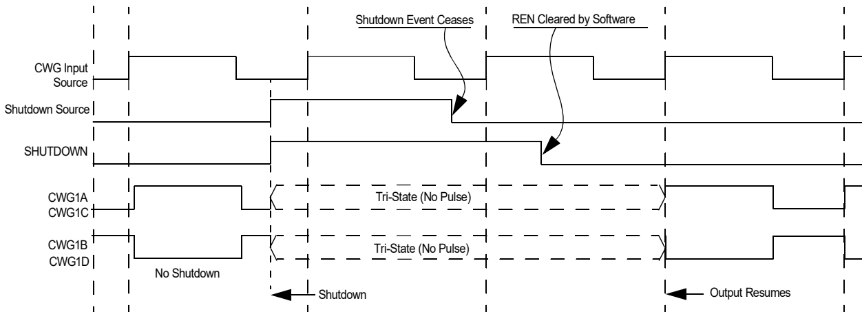
Figure 24-15. SHUTDOWN FUNCTIONALITY, AUTO-RESTART DISABLED (REN = 0, LSAC = 01, LSBSD = 01)
