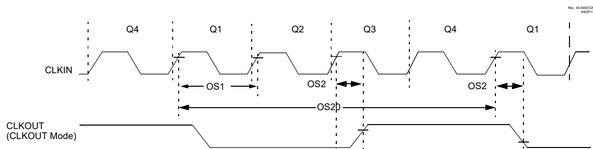
Figure 38-4. Clock Timing
