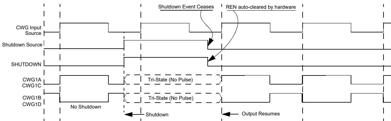
Figure 24-16. SHUTDOWN FUNCTIONALITY, AUTO-RESTART ENABLED (REN = 1, LSAC = 01, LSBD = 01)
