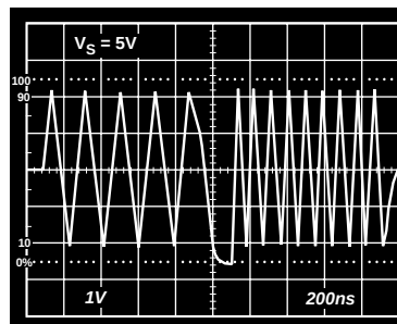
Figure 8. 2:1 Multiplexer Performance
