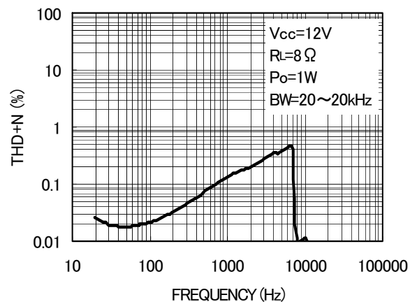
Fig. 2 THD+N — Frequency
