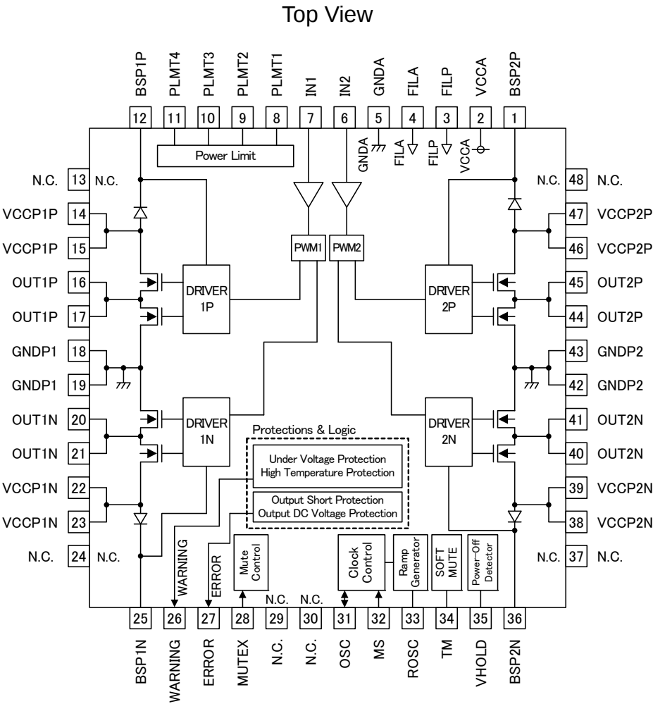
Fig. 28 Pin Assignment Diagram
