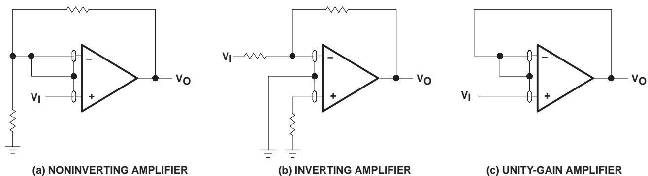
Figure 41. Guard-Ring Schemes
