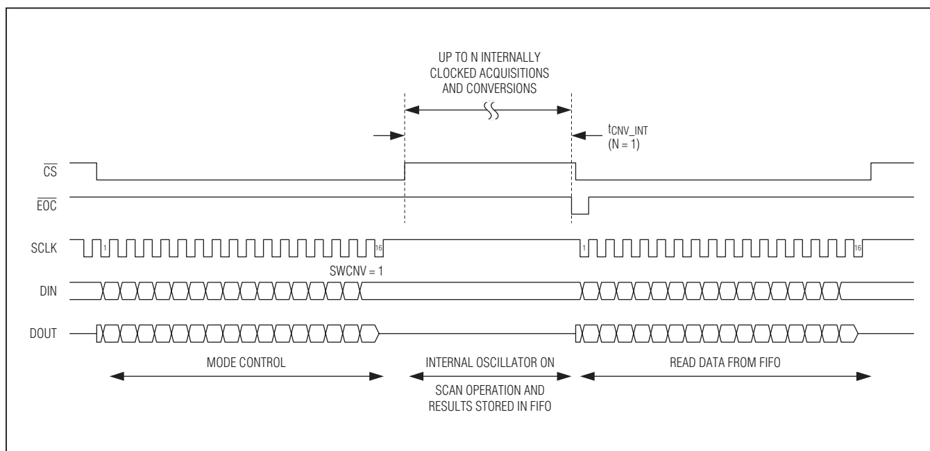
Figure 7. Internal Conversions with \text{SWCNV} ( N = \text{Up to 512 Conversions: } 16 \text{ Channels} \times 32\text{Avg/Channel} = 512 )
