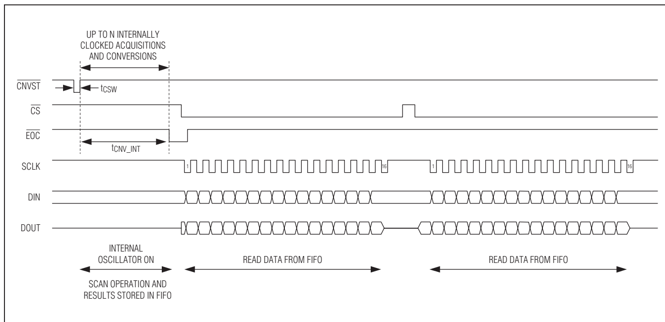
Figure 6. Internal Conversions with \overline{\text{CNVST}} ( N = \text{Up to 512 Conversions: } 16 \text{ Channels} \times 32\text{Avg/Channel} = 512 )
