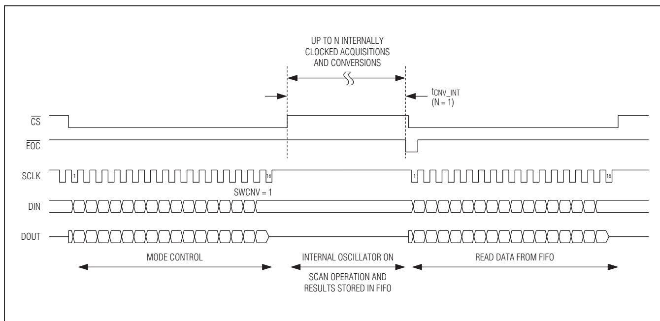
Figure 7. Internal Conversions with SWCNV ( N = \text{Up to 512 Conversions: } 16 \text{ Channels} \times 32\text{Avg/Channel} = 512 )
