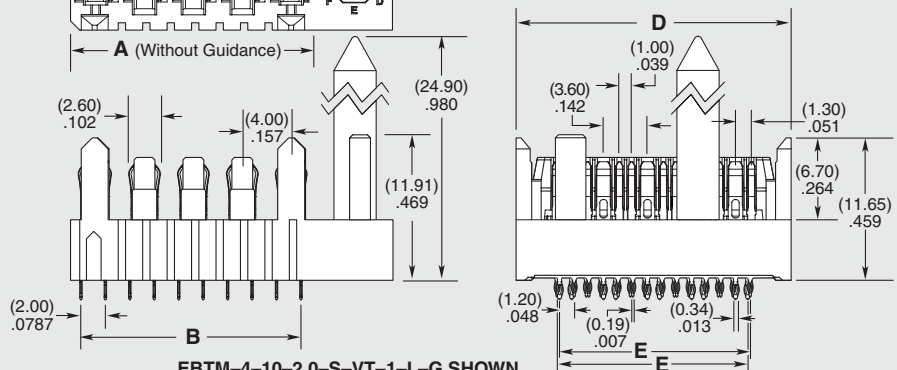
EBTM-4-10-2.0-S-VT-1-L-G SHOWN
