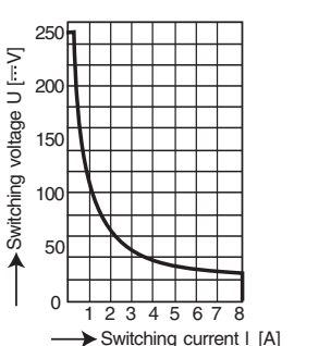
Safe disconnection, no remaining arc, max. 1 operation/sec.
