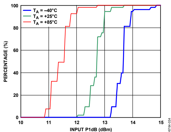
Figure 38. IP1\text{dB} Distributions
