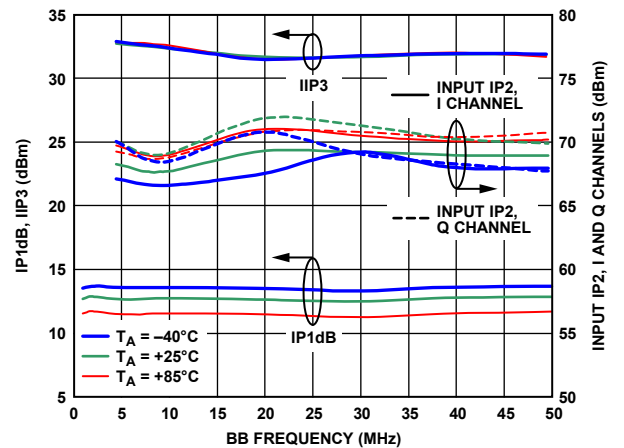
Figure 19. IIP3, IIP2, IP1dB vs. Baseband Frequency
