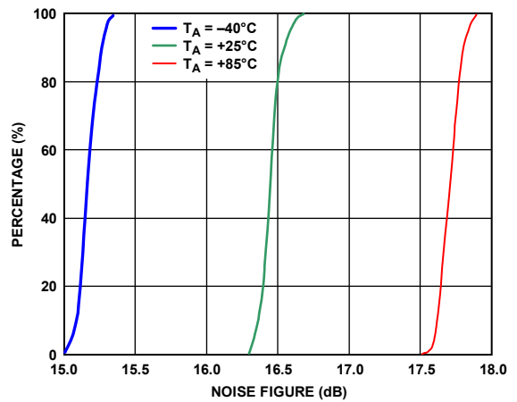
Figure 47. Noise Figure Distributions
