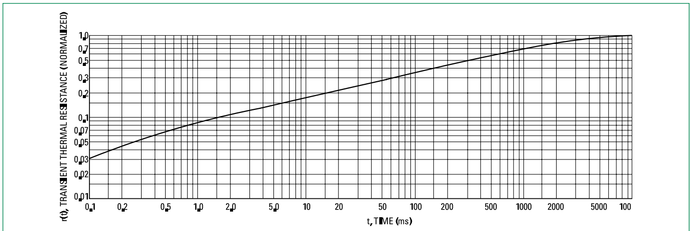
Figure 4. Thermal Response
