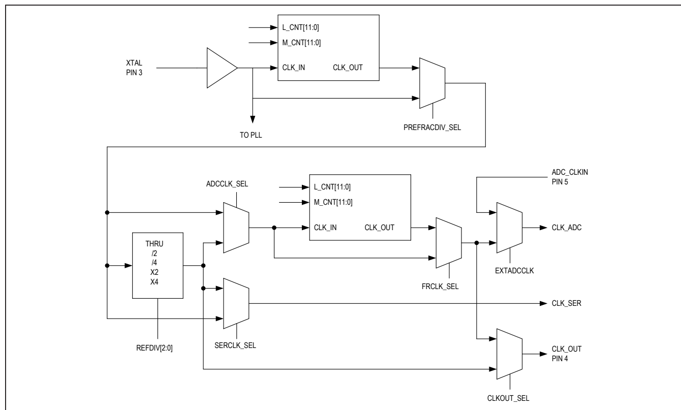
Figure 3. Clock Distribution
