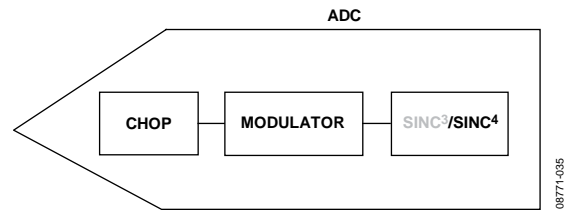
Figure 40. Chop Enabled
