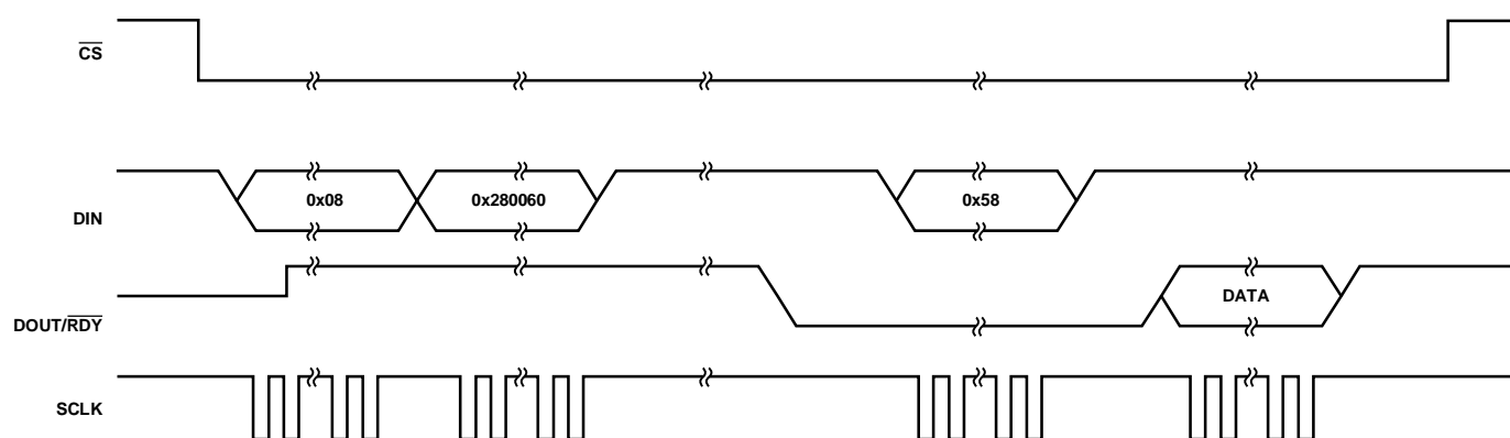
Figure 21. Single Conversion
