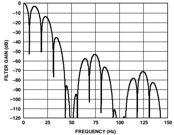
Figure 43. Sinc^4 Filter Response (FS[9:0] = 96, Chop Enabled)
