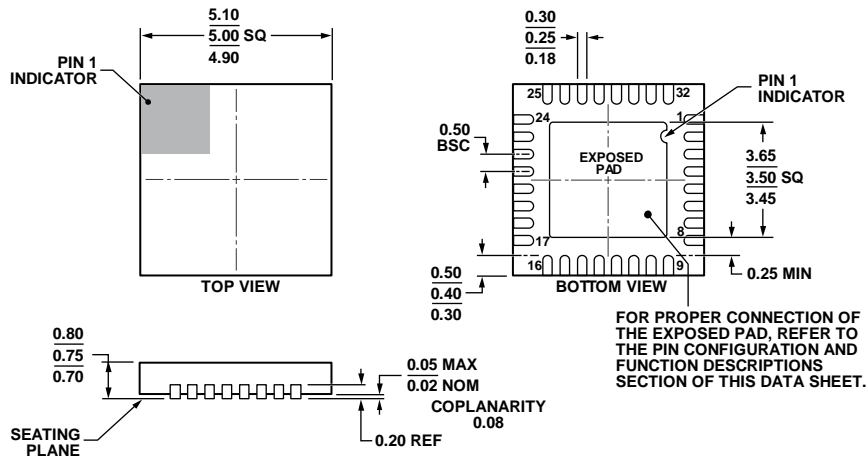
COMPLIANT TO JEDEC STANDARDS MO-220-WHHD. Figure 51. 32-Lead Lead Frame Chip Scale Package [LFCSP-WQ] 5 mm × 5 mm Body, Very Very Thin Quad (CP-32-11) Dimensions shown in millimeters
