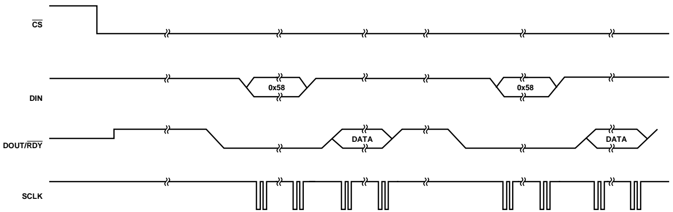
Figure 22. Continuous Conversion
