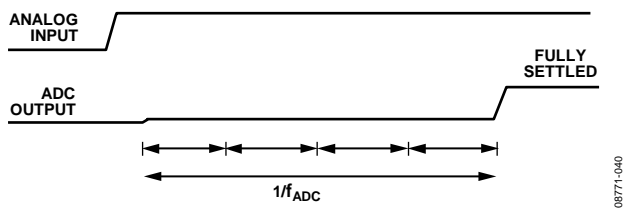
Figure 27. Sinc 4 Zero Latency Operation
