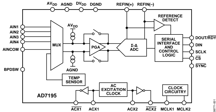
Figure 18. Block Diagram
