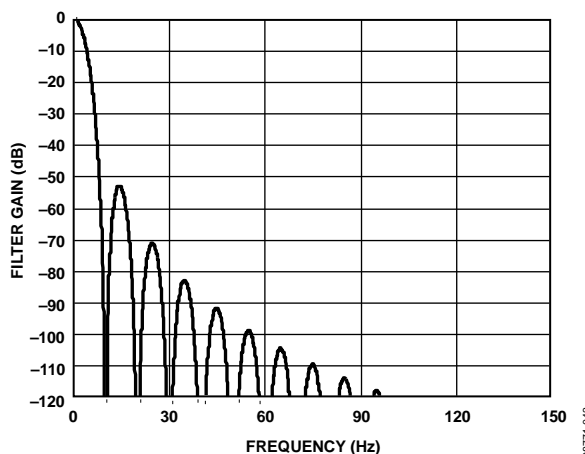
Figure 30. Sinc 4 Filter Response (FS[9:0] = 480)
