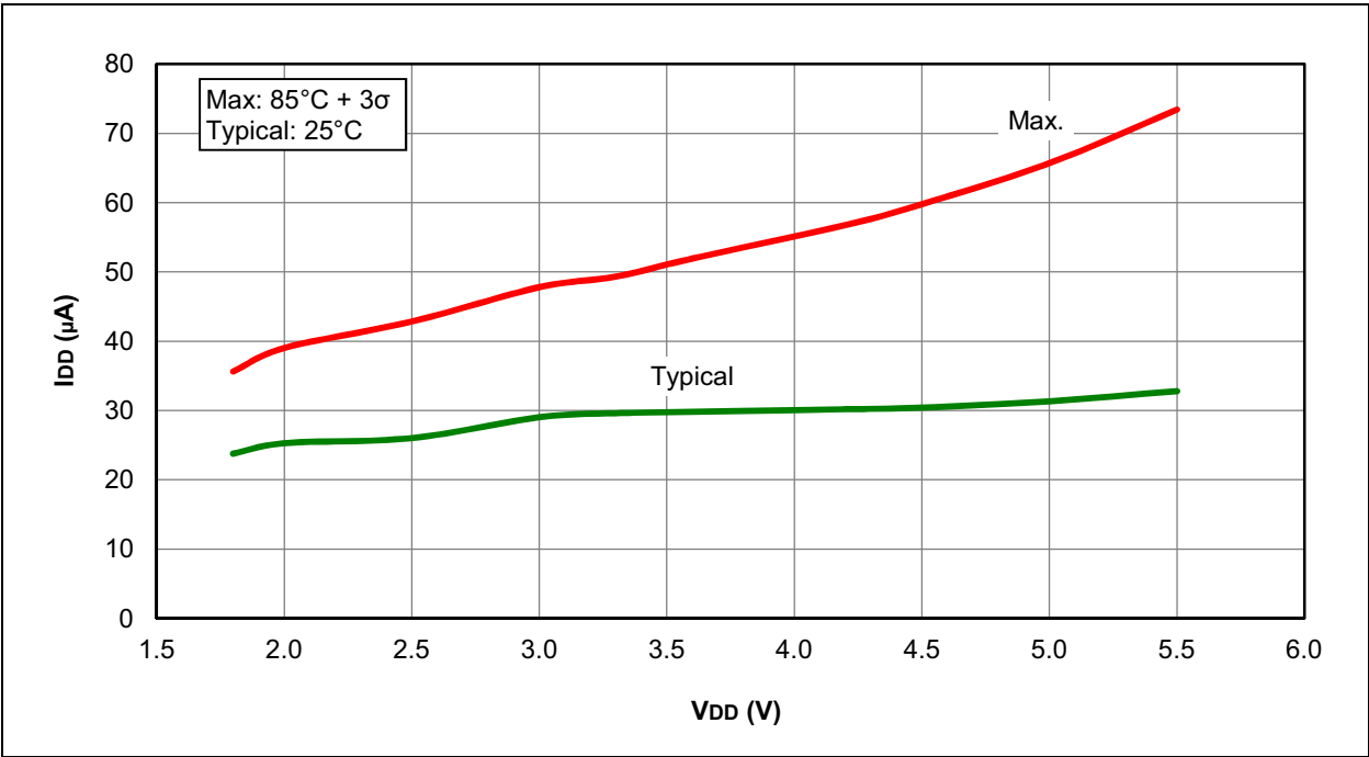
FIGURE 31-2: I_{DD} , LP OSCILLATOR MODE ( F_{osc} = 32\text{ kHz} ), PIC12F1822 AND PIC16F1823 ONLY
