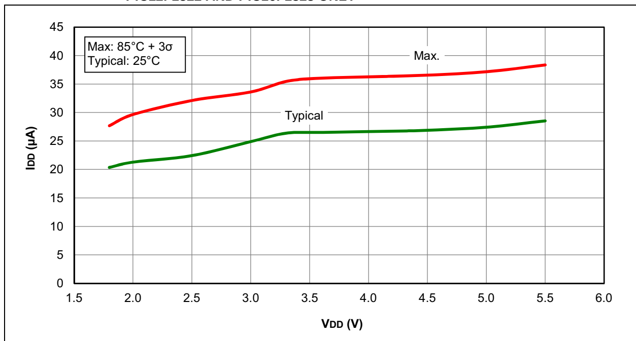
FIGURE 31-8: I_{DD} , EC OSCILLATOR, LOW-POWER MODE ( F_{osc} = 32\text{ kHz} ), PIC12F1822 AND PIC16F1823 ONLY
