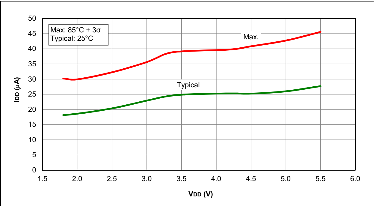
FIGURE 31-10: I_{DD} , EC OSCILLATOR, LOW-POWER MODE ( F_{osc} = 500\text{ kHz} ), PIC12F1822 AND PIC16F1823 ONLY
