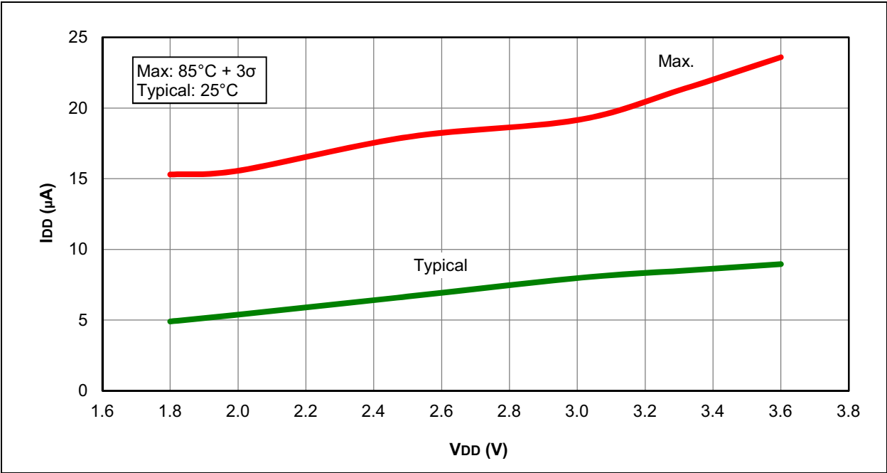
FIGURE 31-1: I_{DD} , LP OSCILLATOR MODE ( F_{osc} = 32\text{ kHz} ), PIC12LF1822 AND PIC16LF1823 ONLY
