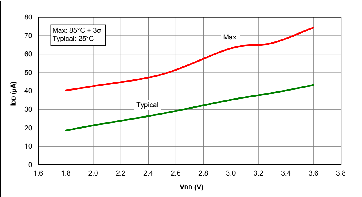
FIGURE 31-9: I_{DD} , EC OSCILLATOR, LOW-POWER MODE ( F_{osc} = 500\text{ kHz} ), PIC12LF1822 AND PIC16LF1823 ONLY
