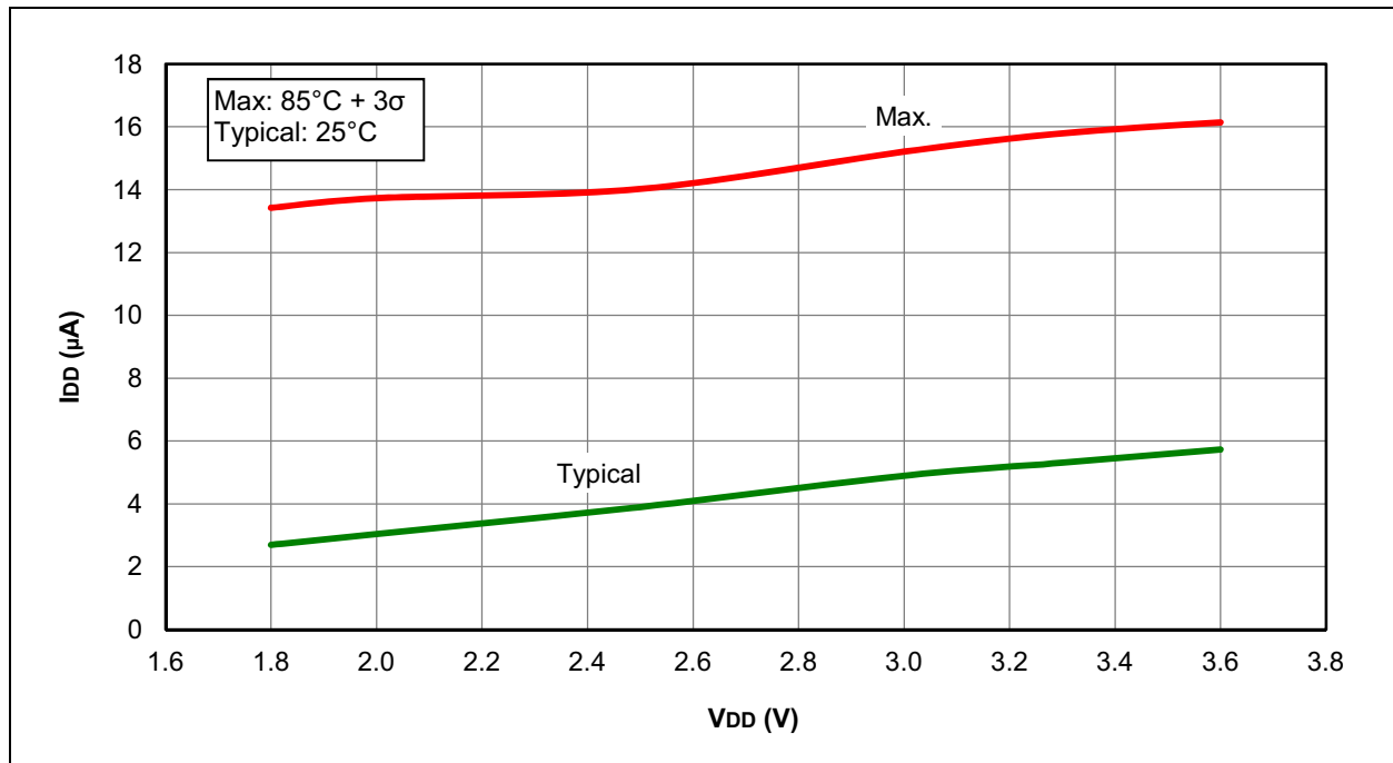
FIGURE 31-7: I_{DD} , EC OSCILLATOR, LOW-POWER MODE ( F_{osc} = 32\text{ kHz} ), PIC12LF1822 AND PIC16LF1823 ONLY
