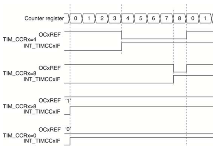
Figure 9.22. Edge-Aligned PWM Waveforms (ARR = 8)
