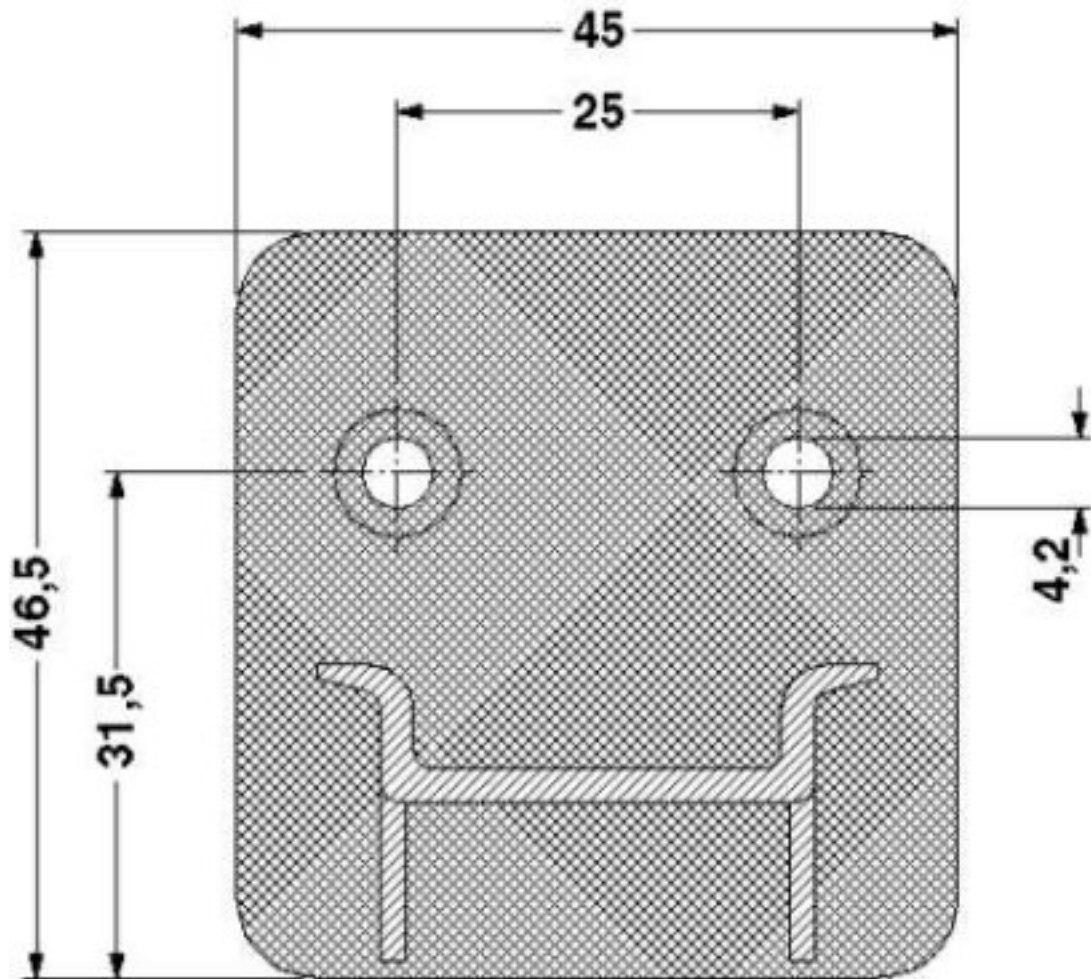
Dimensioned drawing
