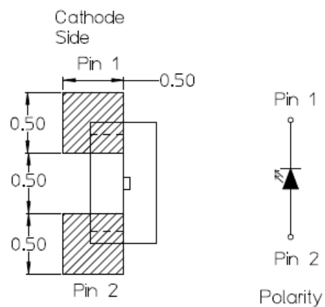
Figure 12: Recommended Solder Pad (Units: mm)
