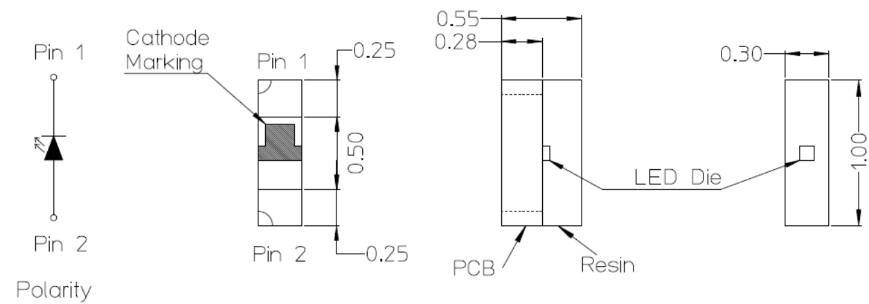
Figure 1: Package Dimensions
