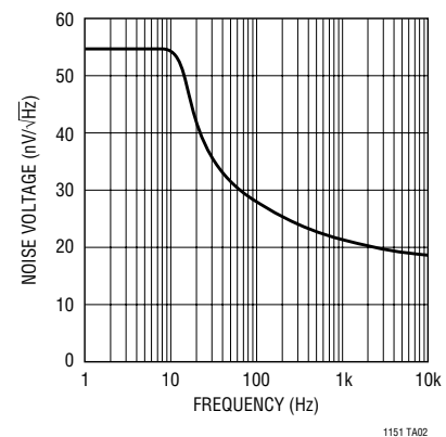
Noise Spectrum
