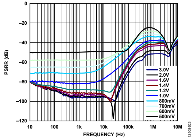
Figure 26. Power Supply Rejection Ratio (PSRR) vs. Frequency, V_{OUT} = 3.3 V , for Various Headroom Voltages
