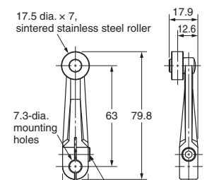
WL-1A300 Lever Length: 63
