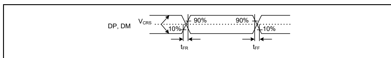
Figure 2.101 DP and DM Output Timing (Full-Speed)
