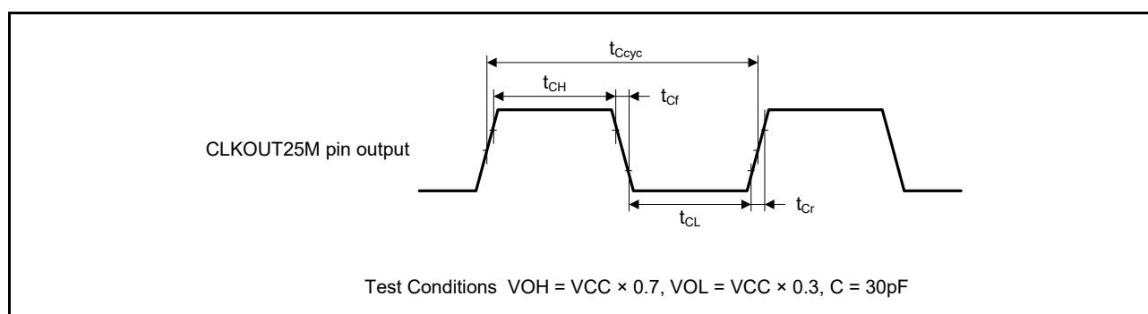
Figure 2.13 CLKOUT25M Pin Output Timing
