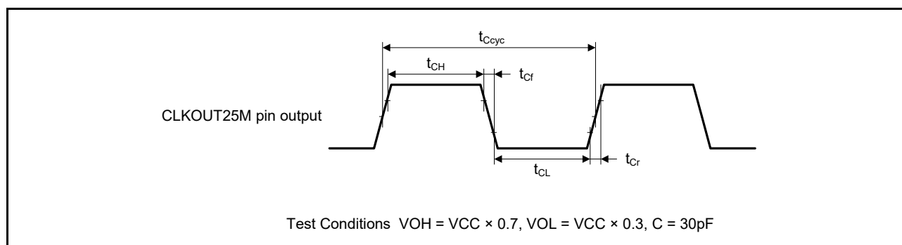
Figure 2.13 CLKOUT25M Pin Output Timing
