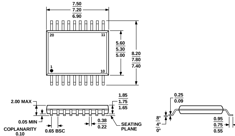
Figure 3. 20-Lead Shrink Small Outline Package [SSOP] (RS-20) Dimensions shown in millimeters
