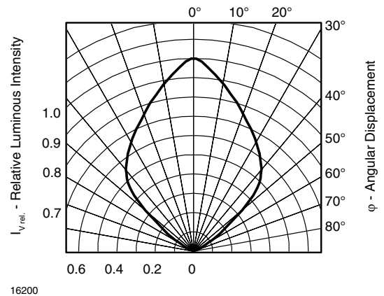
Fig. 3 - Rel. Luminous Intensity vs. Angular Displacement
