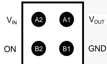
Figure 6. Pin Assignments (Bottom View)
