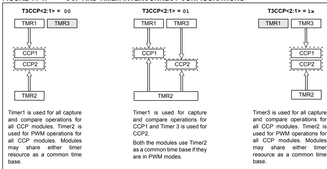
FIGURE 14-1: CCP AND TIMER INTERCONNECT CONFIGURATIONS
