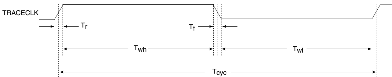
Figure 4. TRACE_CLKOUT specifications
