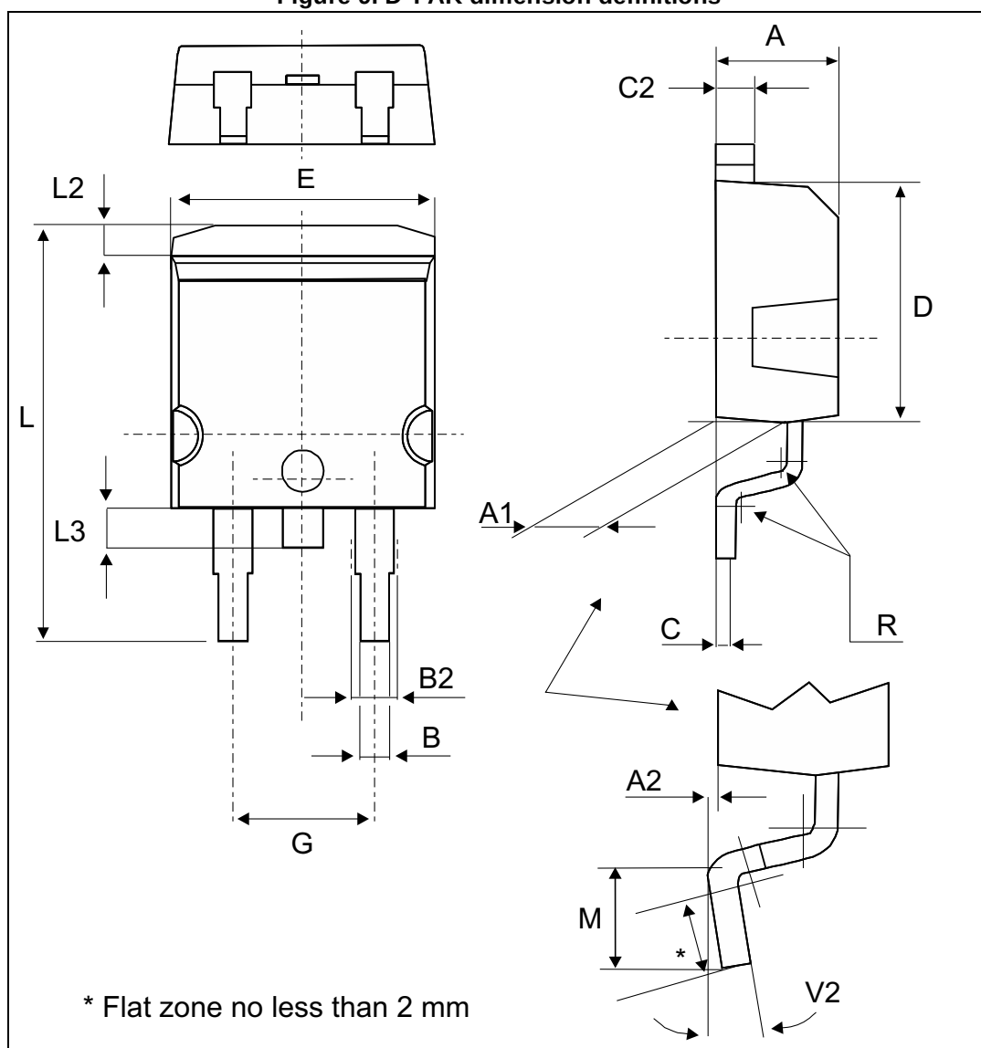
Figure 9. D 2 PAK dimension definitions
