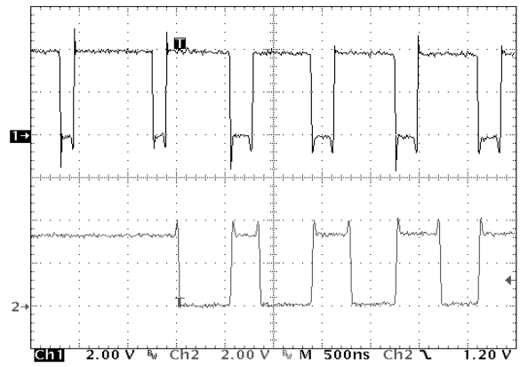
Figure 12. Transitional Period Switch Pins (LX1 and LX2) from Buck to Buck-Boost when V_{IN} - V_{OUT} is > 650 mV
