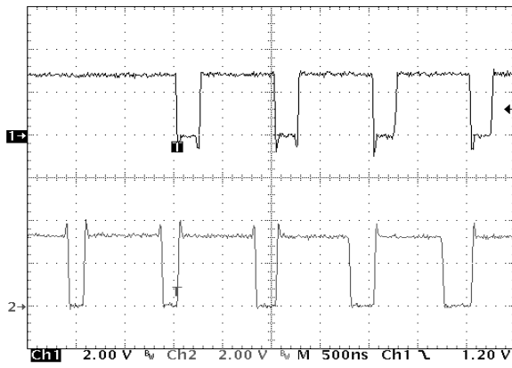
Figure 11. Transitional Period Switch Pins (LX1 and LX2) from Boost to Buck-Boost when V_{OUT} - V_{IN} is < 375 mV
