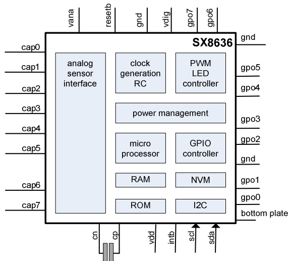
Figure 3 Simplified block diagram of the SX8636
