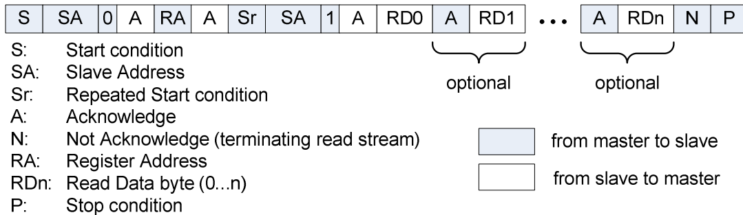
Figure 45 I2C read
