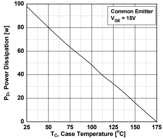
Figure 20. Power Dissipation
