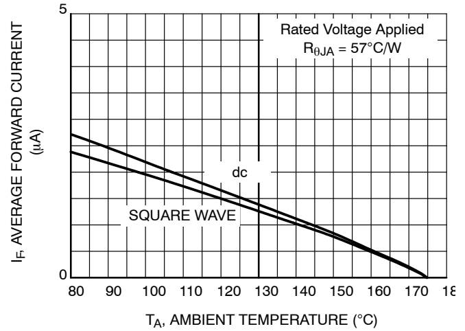
Figure 6. Typical Current Derating, Ambient
