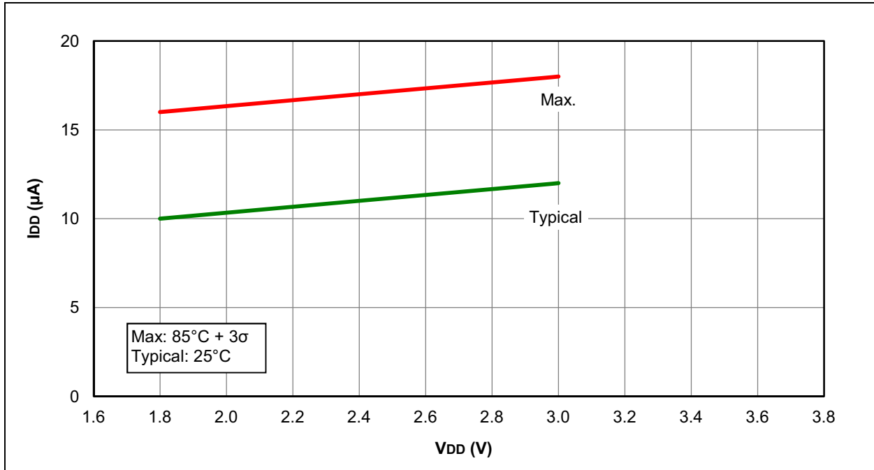
FIGURE 31-11: I_{DD} , LFINTOSC MODE, F_{osc} = 31\text{ kHz} , PIC16LF1847 ONLY
