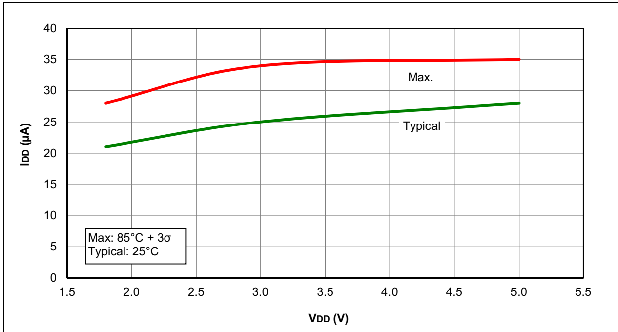
FIGURE 31-12: I_{DD} , LFINTOSC MODE, F_{osc} = 31\text{ kHz} , PIC16F1847 ONLY
