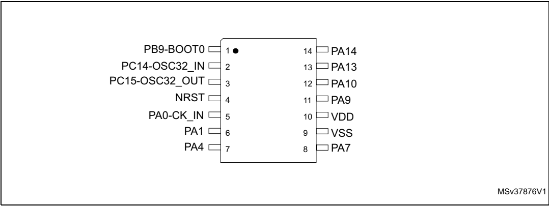
Figure 9. STM32L011x3/4 TSSOP14 pinout
