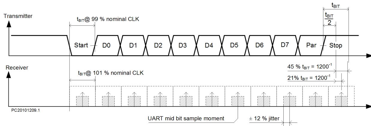
Figure 9. Clock Skew
