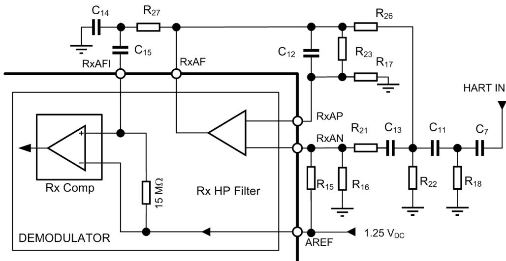
Figure 14. Receive Filter
