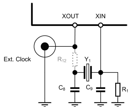
Figure 7. Clock Generation Circuit (External Clock)
