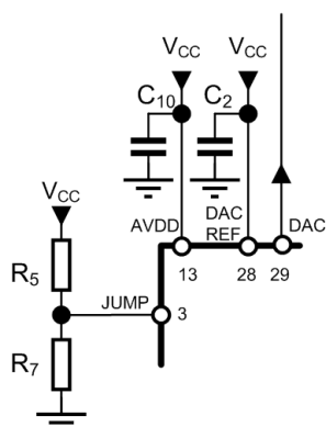
Figure 11. DAC Interface
