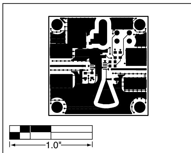
Figure 3. MAX2645 EV Kit PC Board Layout—Component Side
