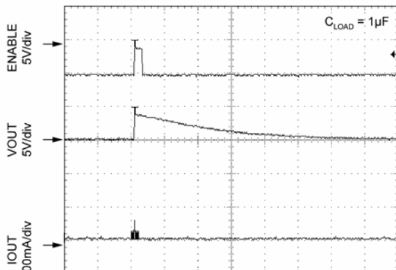
TIME 250µs/div
