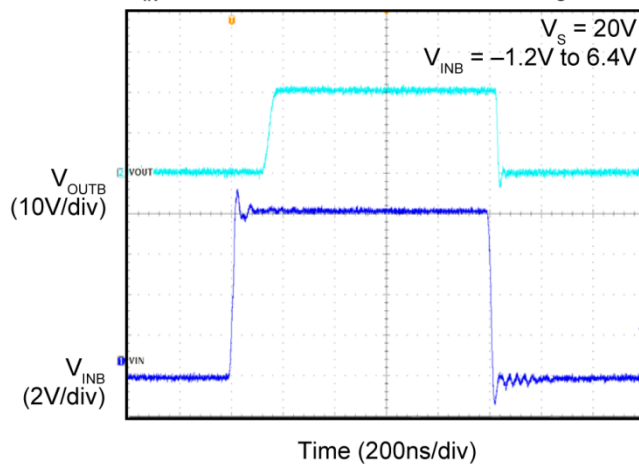
V_{IN} Positive and Negative Input - V_S = 20V
