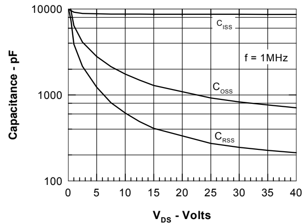
Figure 8. Capacitance Curves
