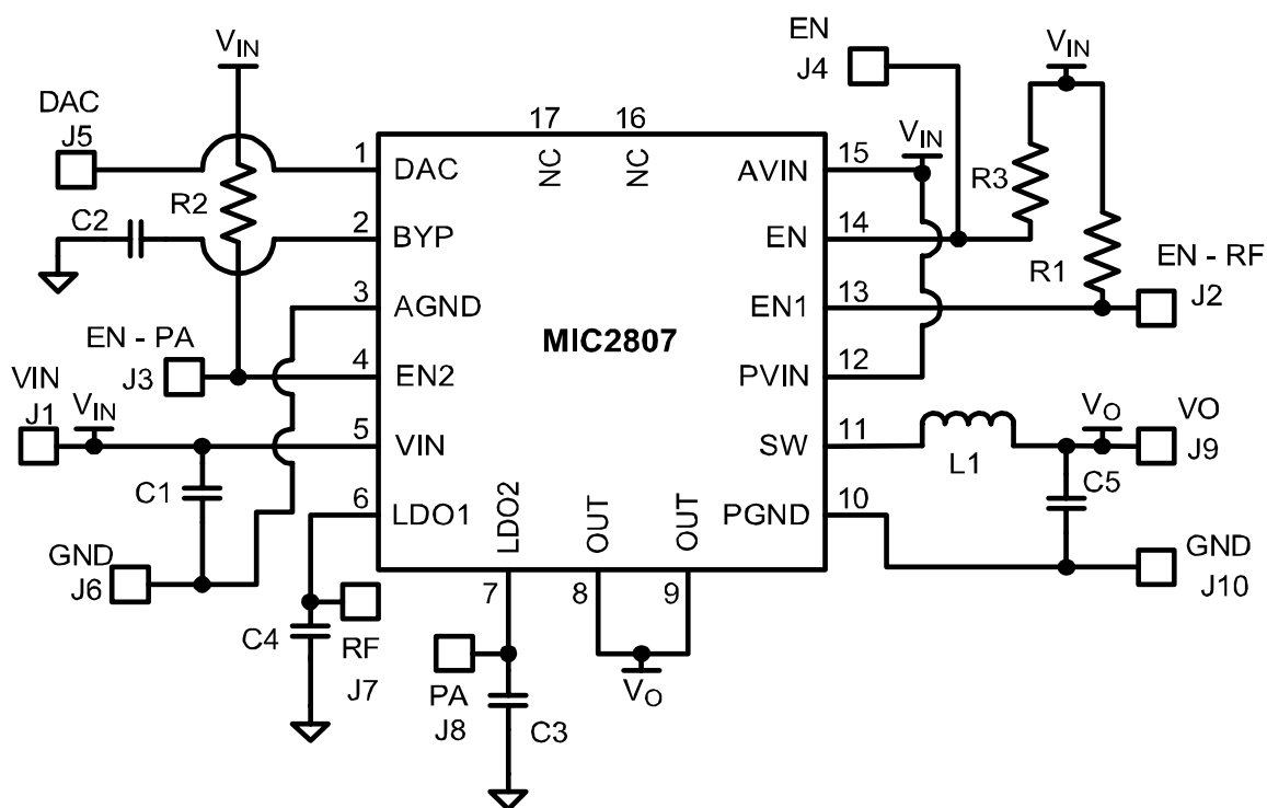
Layout Schematic
